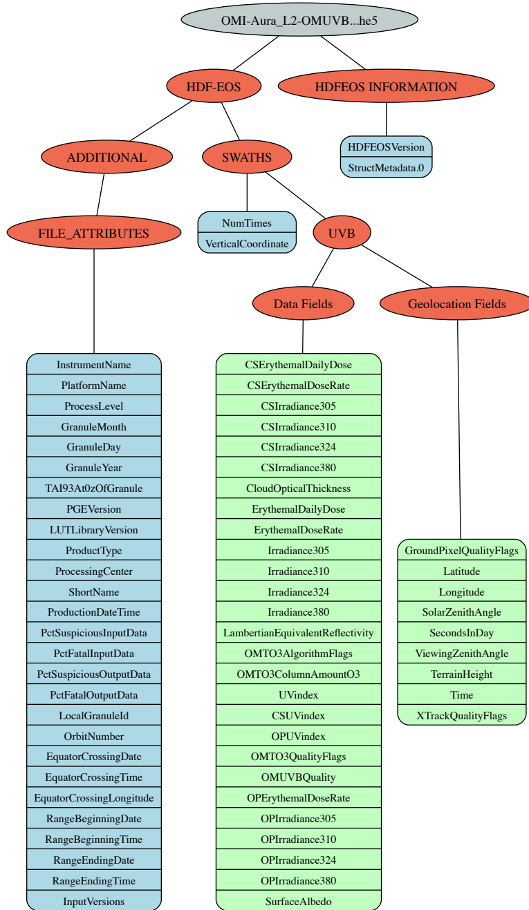
Figure 1: Structure of the OMUVB product file. Colors indicate groups (red), attributes (blue) and datafields (green).
